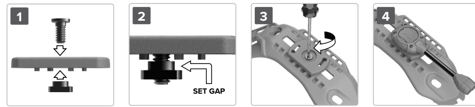
Figure 7 – MICH Mount Installation
